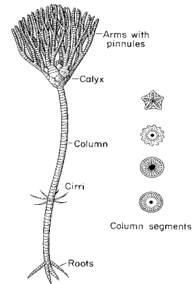
Crinoid
