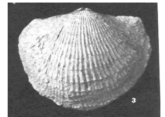
Brachiopods
