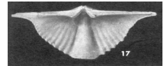
Brachiopods
